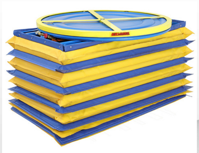
Above - EZ Loader on the Portability Kit Below - Fitted Safety Skirting
